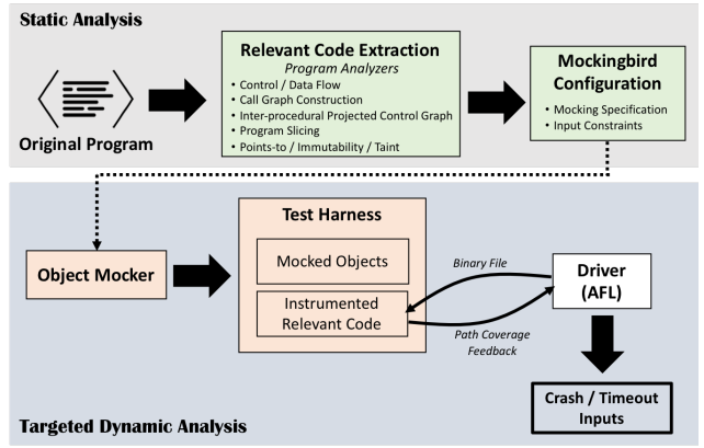
Fig. 1. Mockingbird Framework Architecture and Workflow
